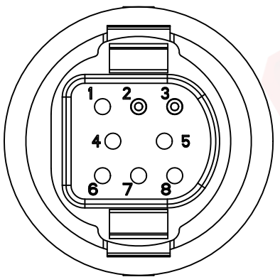
Pin Hole View Scale:2/1
